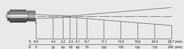
CF-Optik, D:S = 22:1 (Fernfeld = 6:1)
