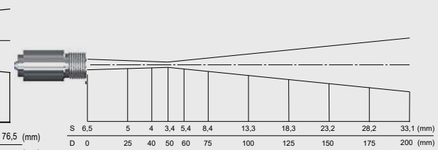
CF-Optik, D:S = 15:1 (Fernfeld = 5:1)
