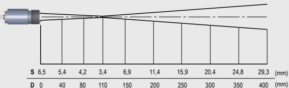
Optik CSmicro 3MH CF, D:S = 33:1 (Fernfeld 11:1)
