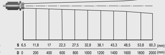
Optik CSmicro 3MH CF, D:S = 33:1 (Fernfeld 11:1)
