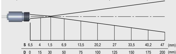
Optik CSmicro 3ML CF1, D:S = 22:1 (Fernfeld 3,5:1)
