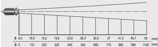
Optik CSmicro 3ML CF, D:S = 22:1 (Fernfeld 9:1)
