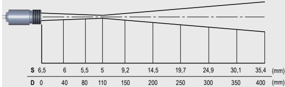
Optik CSmicro 3ML CF, D:S = 22:1 (Fernfeld 9:1)
